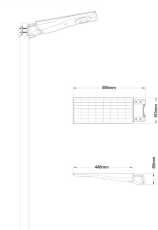
HS-20W-SSL | FIGURE DIMENSION
