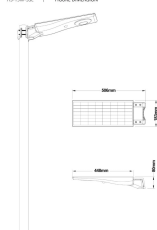
HS-20W-SSL | FIGURE DIMENSION
